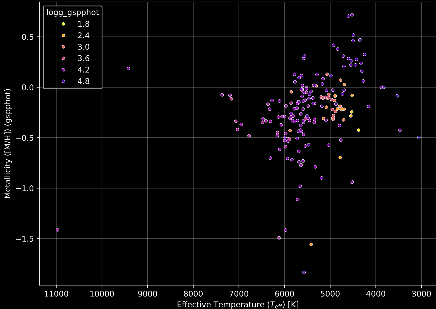
APOGEE DR17 Field: [167+34_MGA] Stellar Population Parameters (n= 182)
