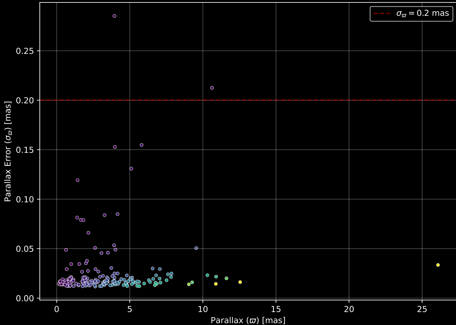
APOGEE DR17 Field: [167+34_MGA] Parallax Quality (n= 182)
