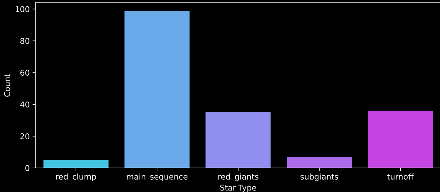
APOGEE DR17 Field: [167+34_MGA] Count plot of Star Type
