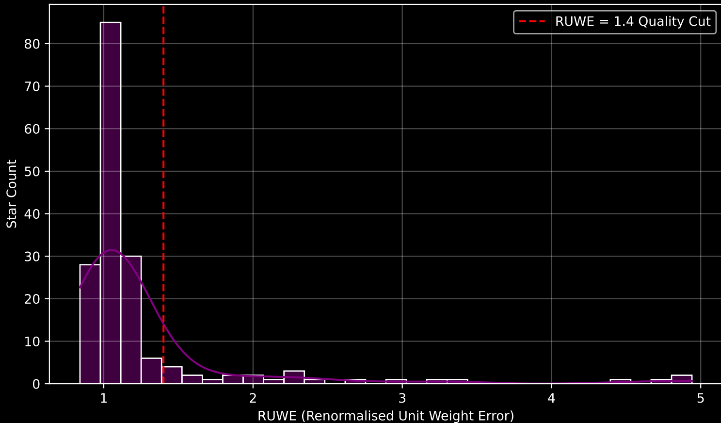
GAPOGEE DR17 Field [167+34_MGA] RUWE Distribution (n= 173)
