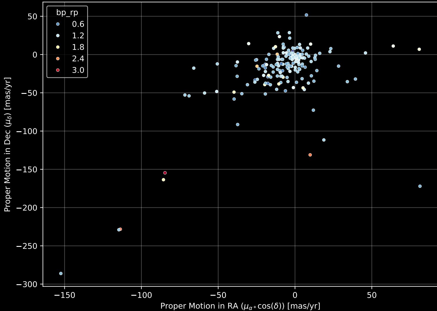
APOGEE DR17 Field: [167+34_MGA] Proper Motion Diagram (n= 182)
