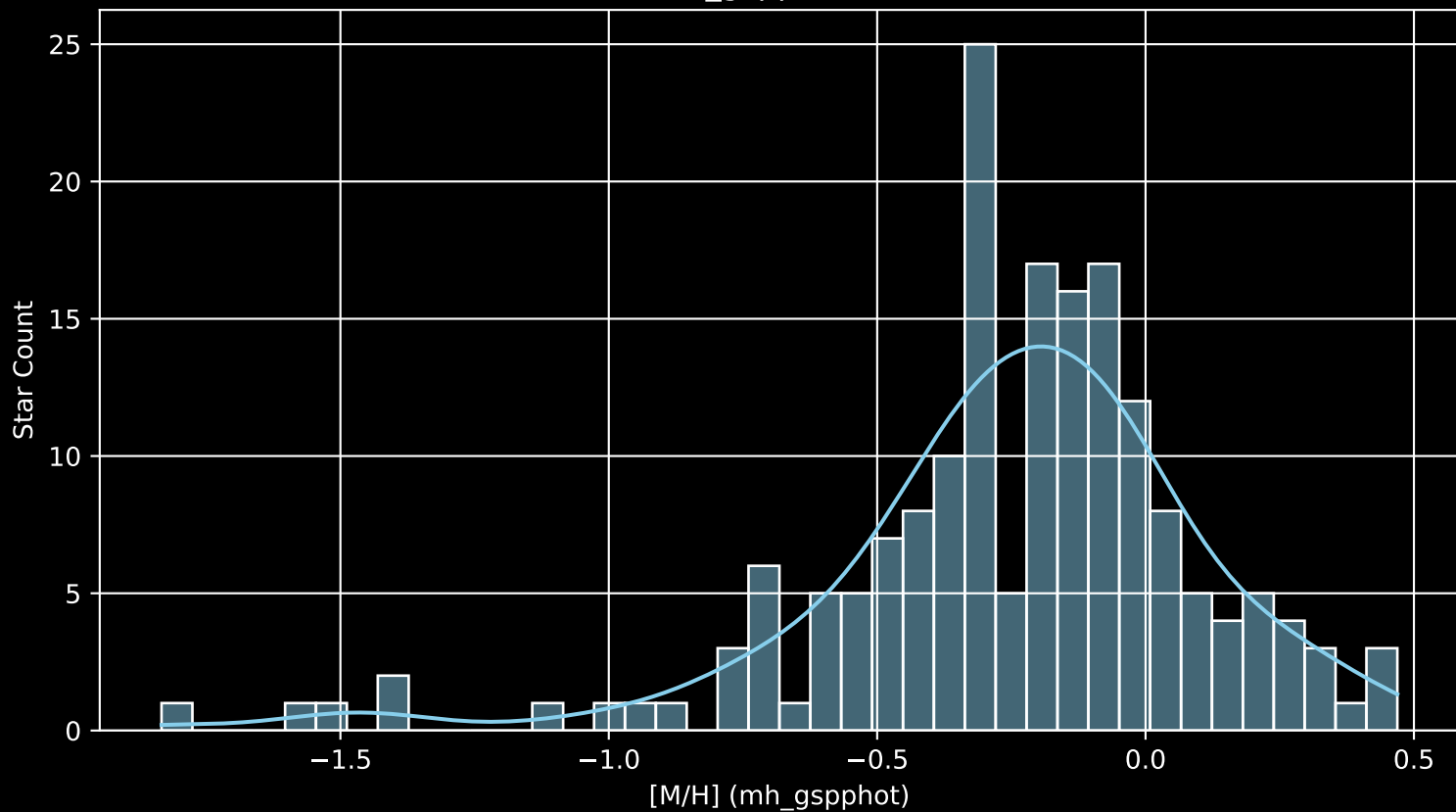
APOGEE DR17 Field: [167+34_MGA [M/H] (mh_gspphot) (n= 179)
