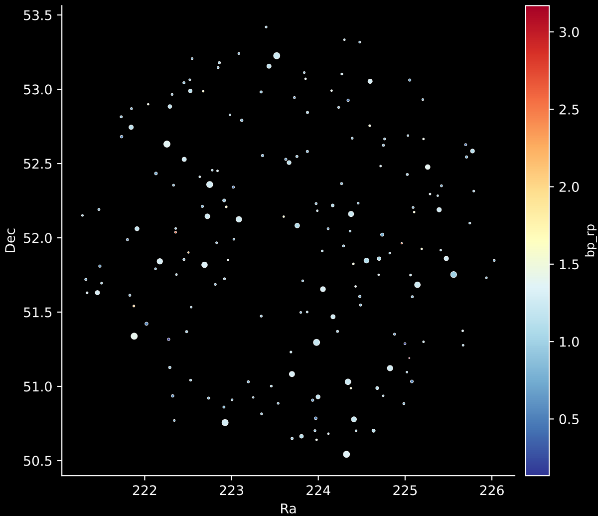
APOGEE DR17 Field: [167+34_MGA] Stars: 182
